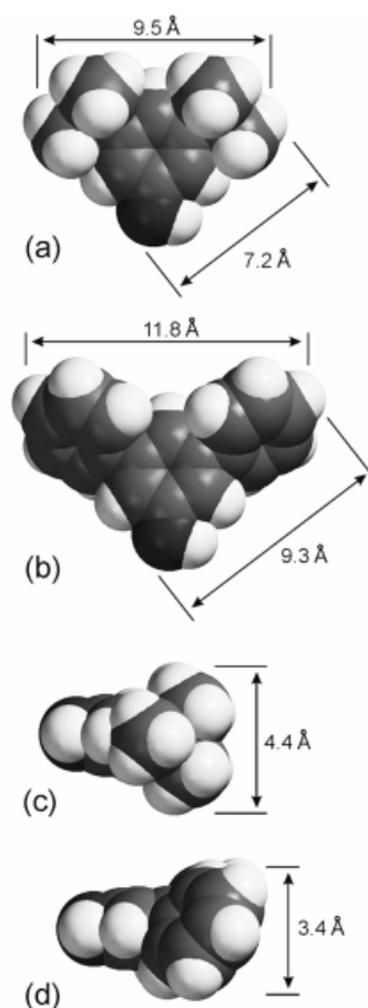
Figure 3. Top (a, b) and side (c, d) views of space-filling models of the 3,5-di- tert -butylphenyl and 3,5-diphenylphenyl stoppers generated with the Sybyl force field. The dimensions given for each stopper are those measured between the centers of the corresponding hydrogen atoms
