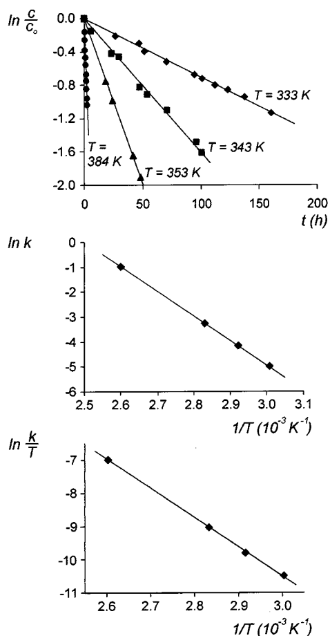
Figure 2. From top to bottom: (a) Determination of rate constants for Rot1@2 at four different temperatures, (b) Arrhenius plot for the evaluation of E_A and k_\infty . (c) Eyring plot for the determination of \Delta G^\ddagger , \Delta H^\ddagger , and \Delta S^\ddagger .
